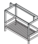
FOUR-POSTER HUT BED H 192 x W 207 x D 102 Ground clearance below the bed 25 CM
